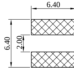
( PCB Pattern )
