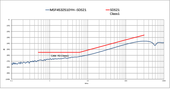
( 3 ) S_{ds21} Curve
