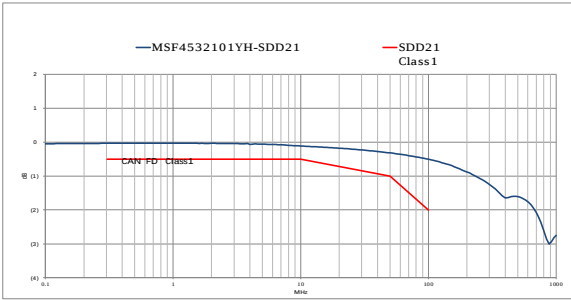
( 1 ) S_{dd21} Curve
