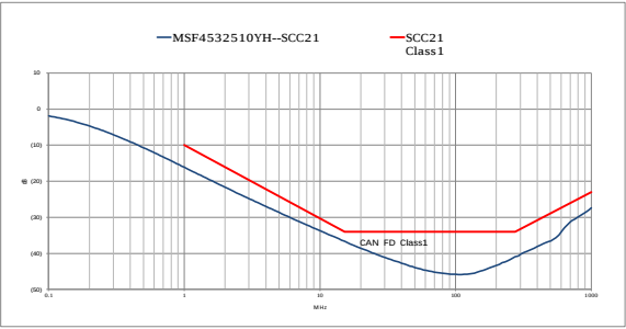
( 2 ) S_{cc21} Curve
