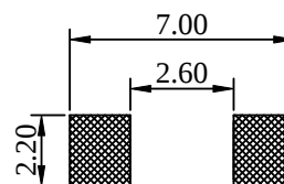
( PCB Pattern )
